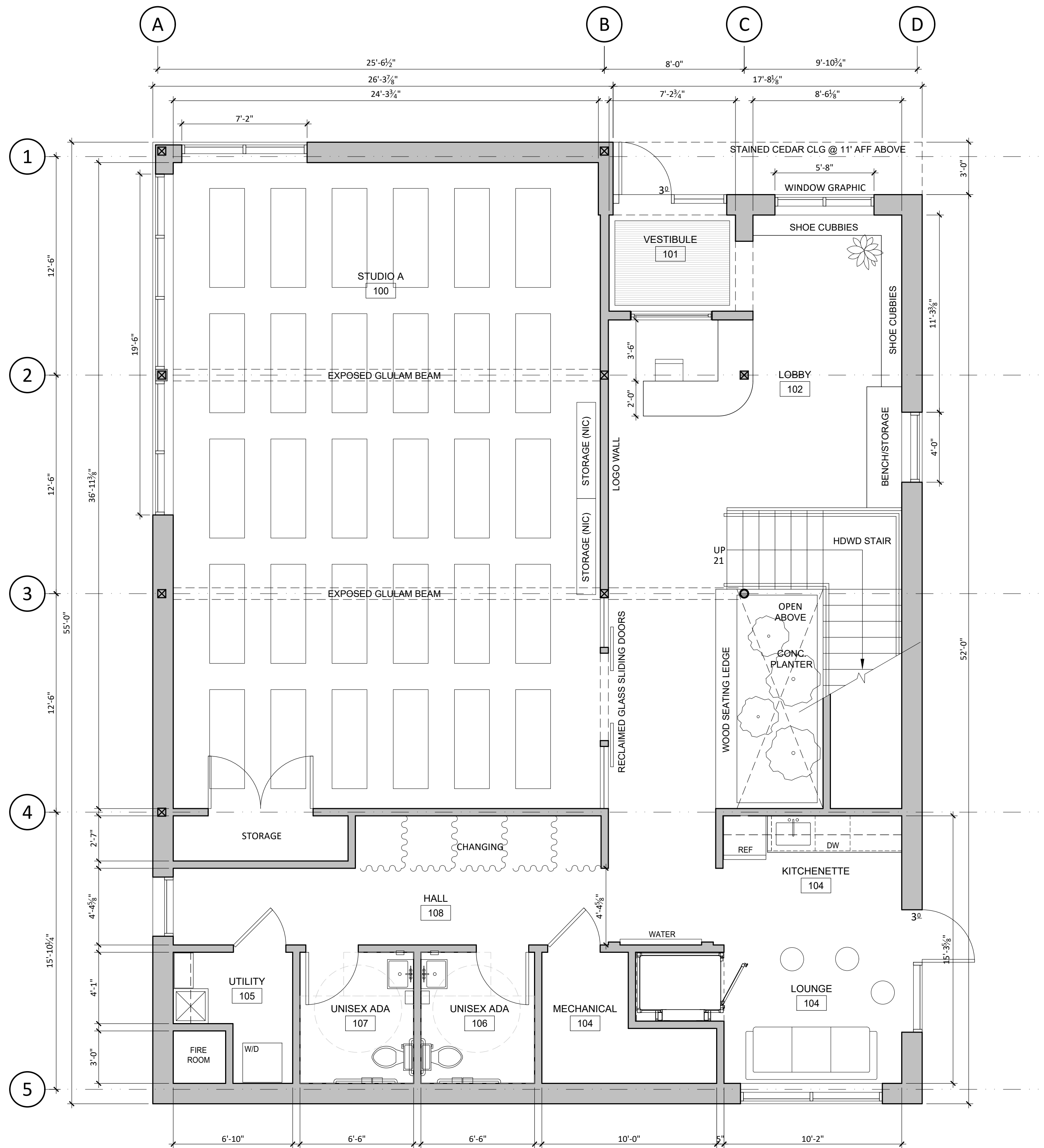
1 PROPOSED MAIN LEVEL PLAN
