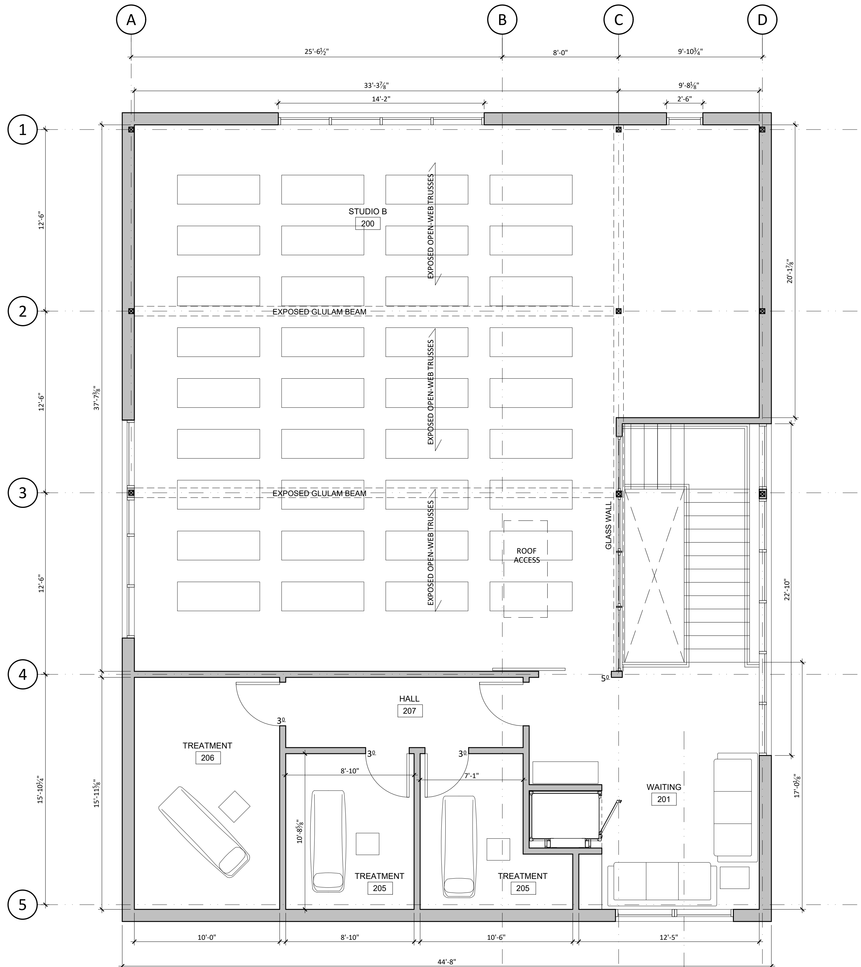
1 PROPOSED SECOND LEVEL PLAN A2.2 1/4" = 1'-0"
